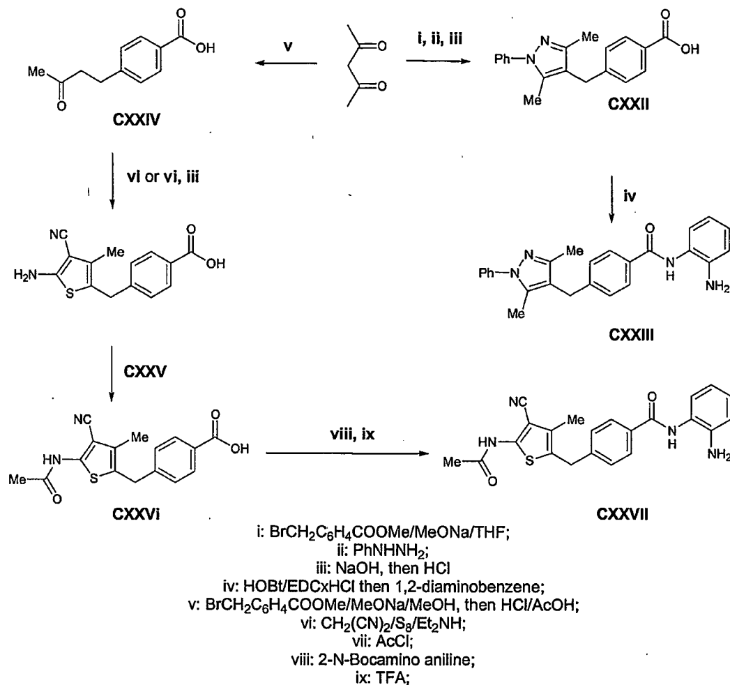
Scheme 49
